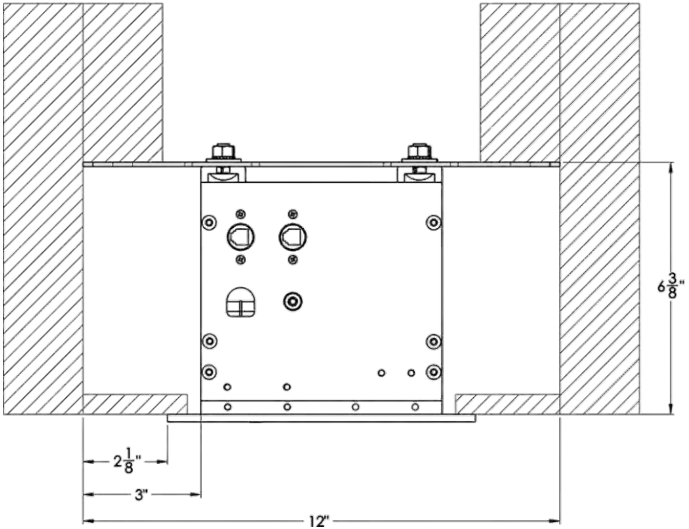
Figure 12. Wing-Out Mount detail with minimum clearance
