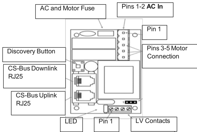
Figure 29. IMC control board schematic
