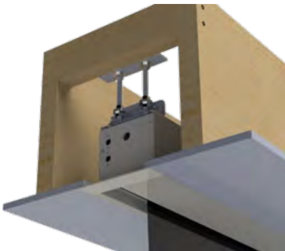
Figure 8. Cascade mounted on ceiling with Threaded Rod Mount
